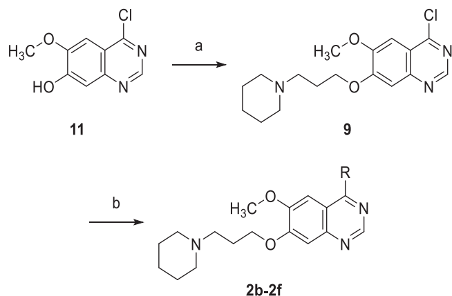
Scheme 2. : Reagents and conditions: (a) 3-piperidin-1-ylpropan-1-ol (1.25 equiv), \text{PPh}_3 (1.3 equiv), DBAD (1.3 equiv), THF, rt, 20 h, > 99%; (b) amines (2.0–10 equiv), DIEA (3.0 equiv), i -PrOH, microwave: 200 W, 160 °C, 15–60 min, 2b : 93%, 2c : 78%, 2d : 89%, 2e : 25%, 2f : 93%.
